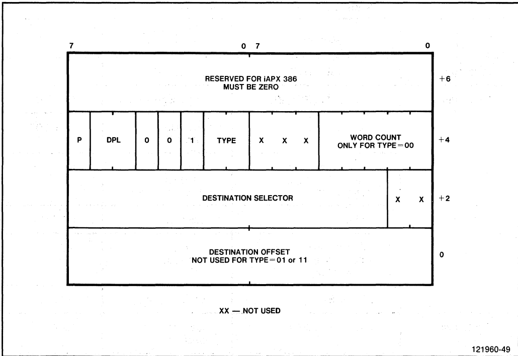
Figure 2-6. Gate Descriptor
