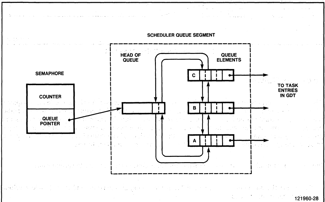
Figure 5-4. Semaphore Structure
