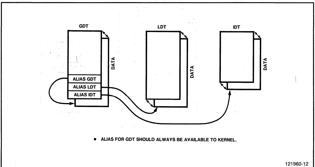
Figure 2-12. Aliases for System Tables
