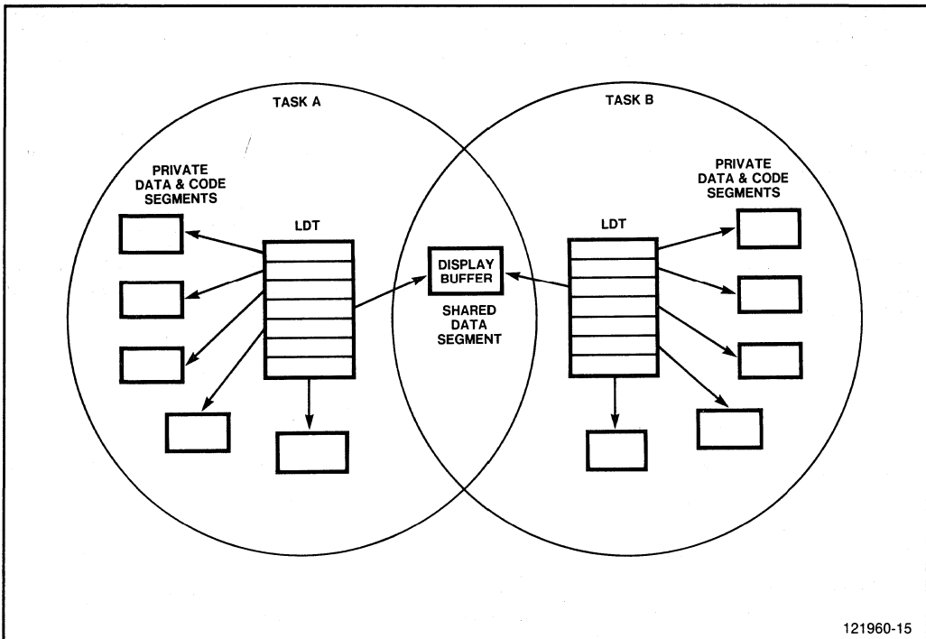
Figure 2-15. Aliases for Segment Sharing
