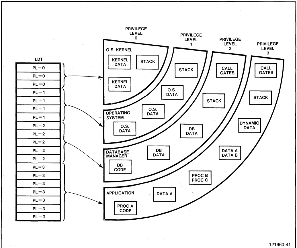
Figure 1-3. Segment Segregation by Privilege Level within a Task
