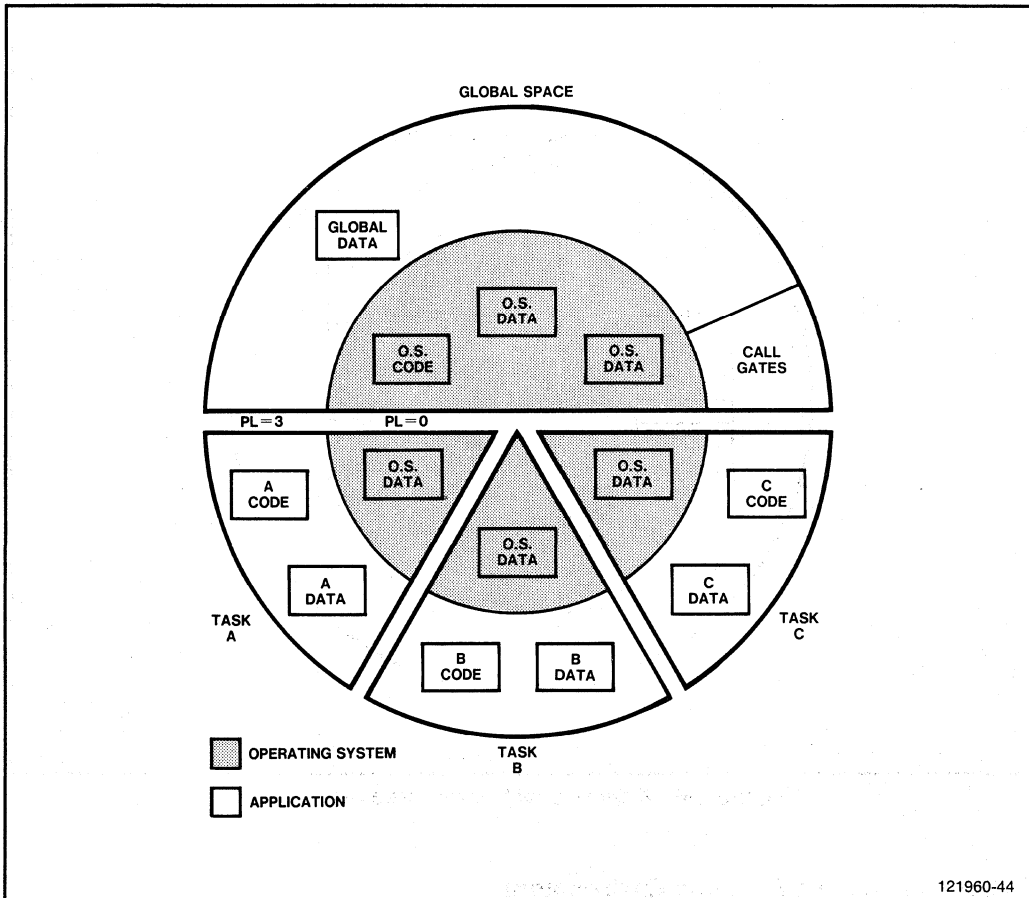
Figure 1-5. A Two-Level Protection Structure
