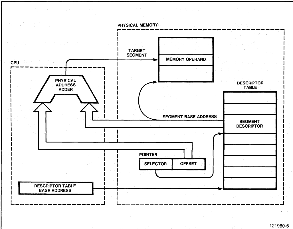
Figure 2-1. Abstraction of Addressing Mechanism
