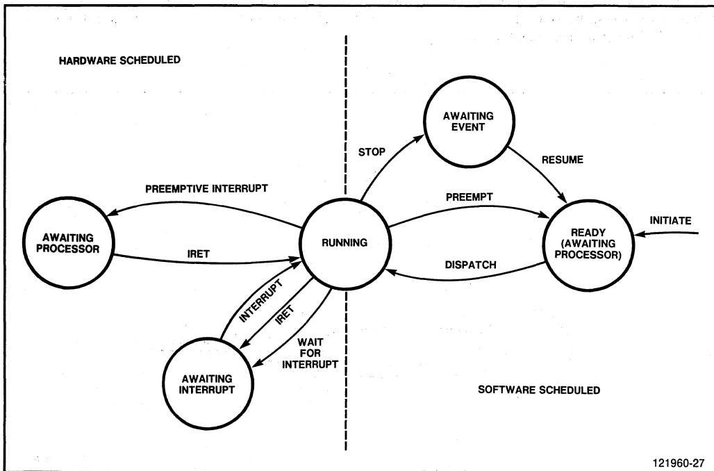
Figure 4-3. Expanded Scheduling State Transition Diagram
