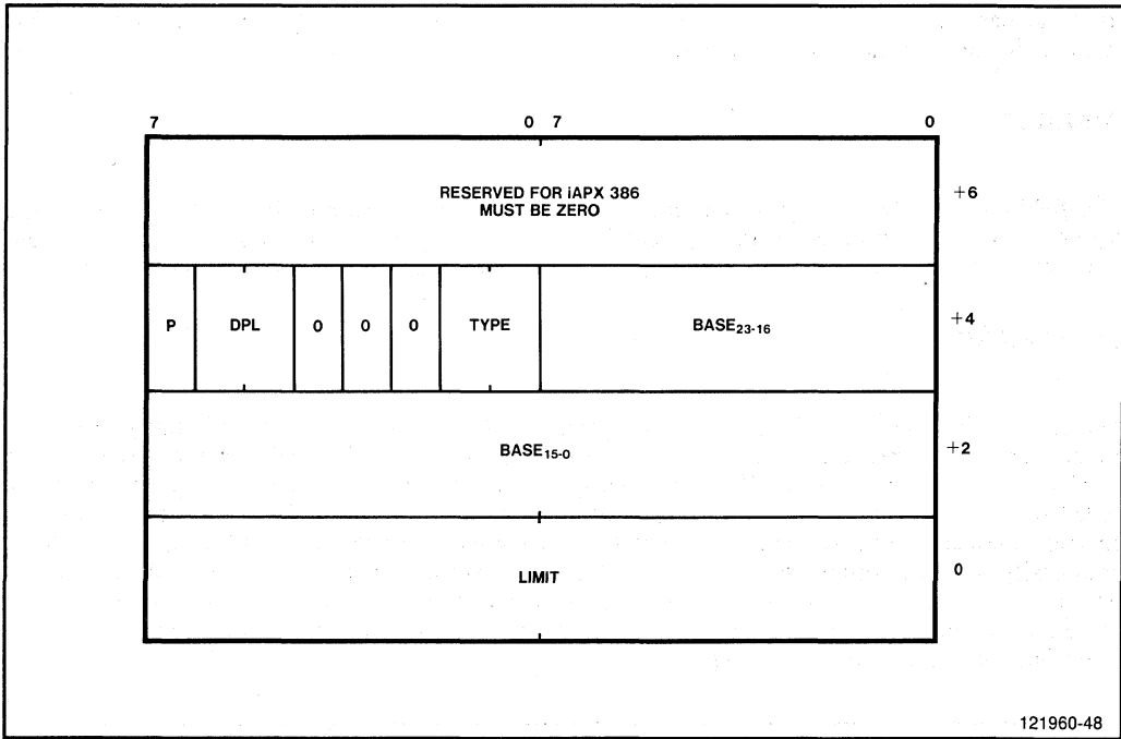
Figure 2-4. System Segment Descriptor
