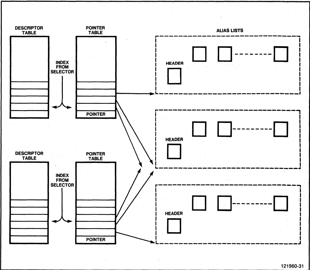
Figure 5-3. Identifying Alias List
