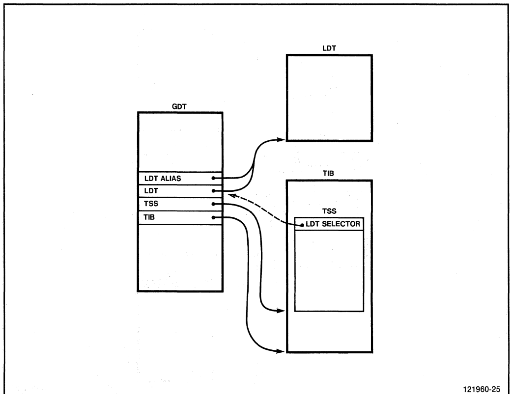
Figure 4-6. Task Information Structure B
