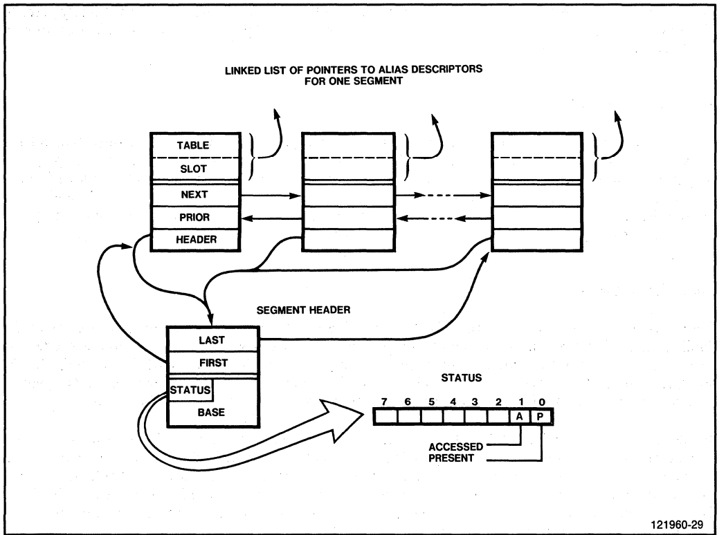
Figure 5-2. Alias List
