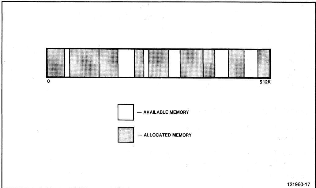
Figure 3-1. Memory Fragmentation
