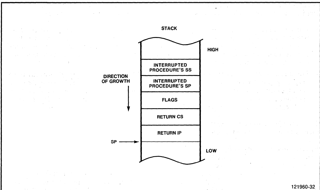
Figure 13-1. Caller's CPL
