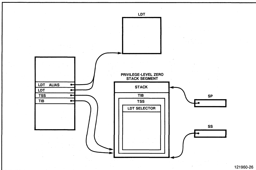
Figure 4-7. Task Information Structure C
