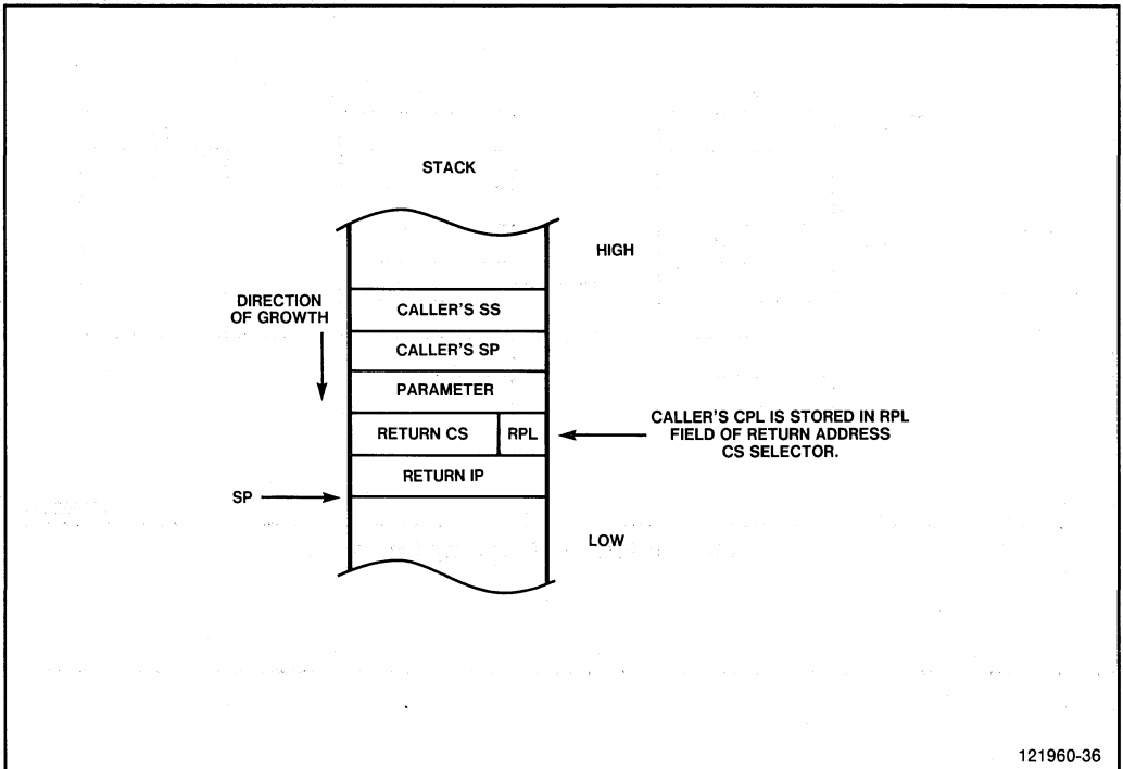
Figure 6-3. Interrupt Procedure's Stack
